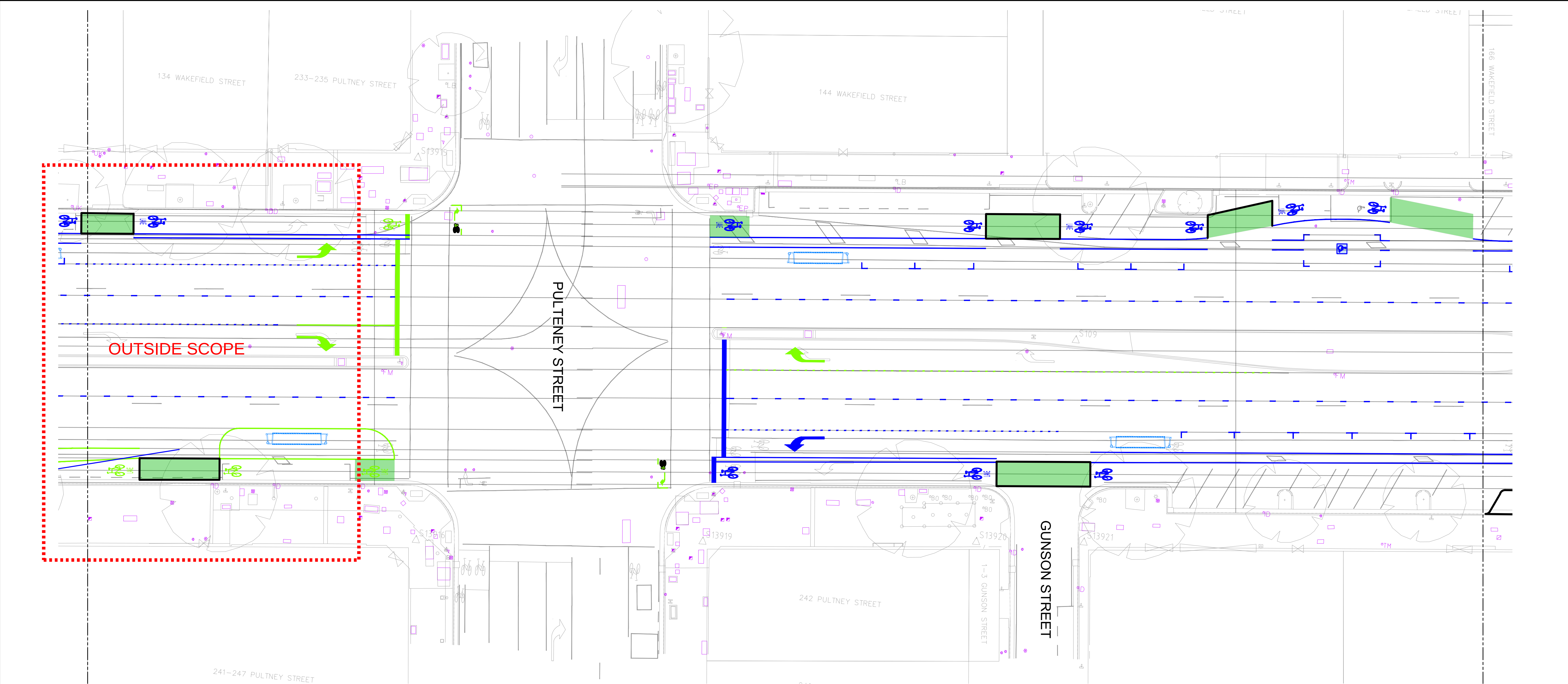
LAYOUT 4 SCALE 1:200
